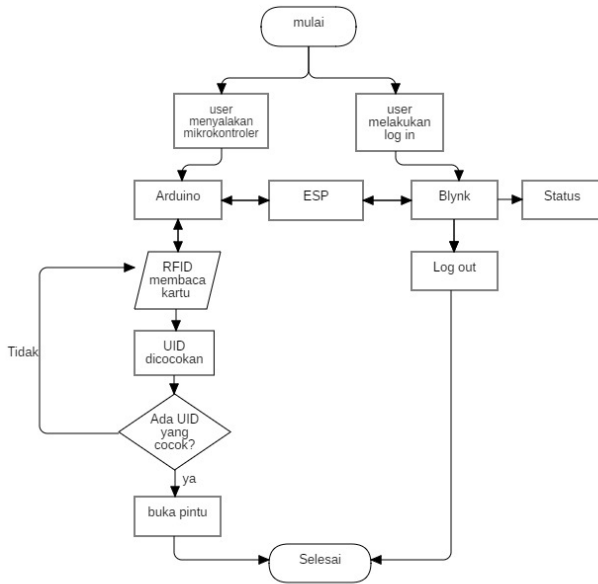
Figure 3.2 Main Program Flowchart
