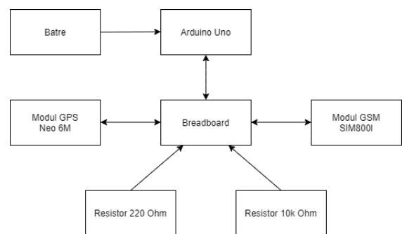
Figure 3.1 System Blok Diagram
